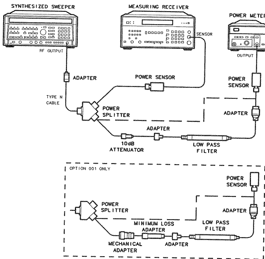
Figure 3-12. LPF Characterization
