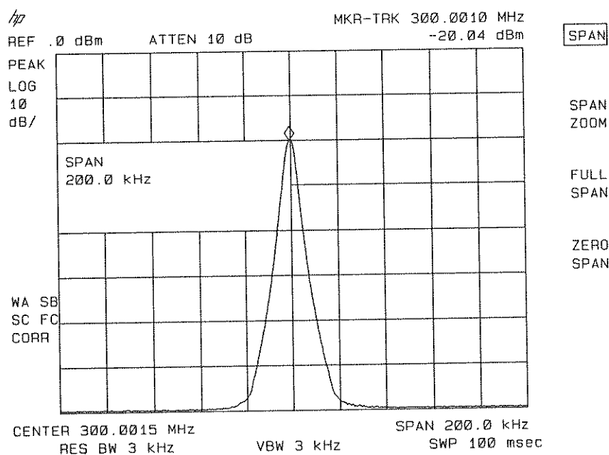
Figure 6-7. After Zooming In on the Signal
