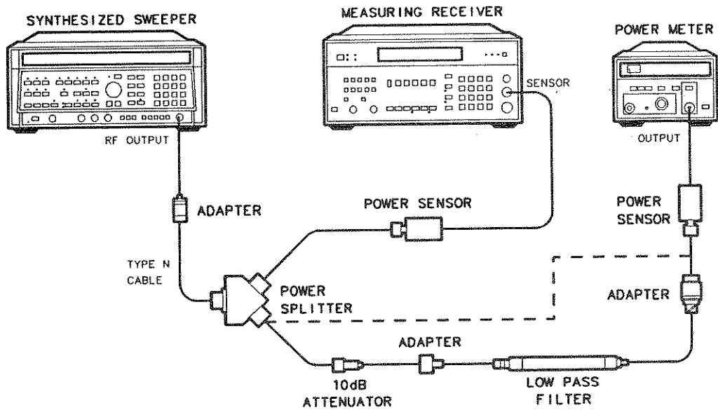
Figure 4-14. LPF Characterization
