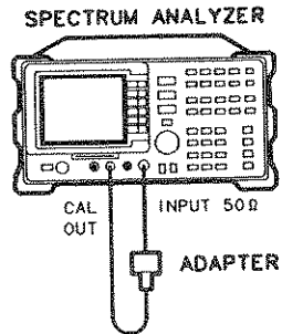
Figure 3-24. Fast Sweep Time Amplitude Test Setup
