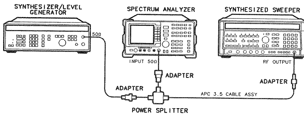
Figure 4-8. Frequency Span Accuracy Test Setup (Spans < 500 MHz)
