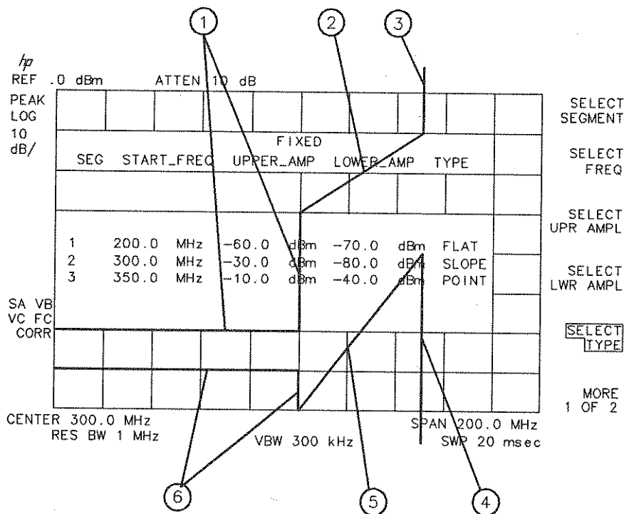
Figure 5-10. Segment Types
