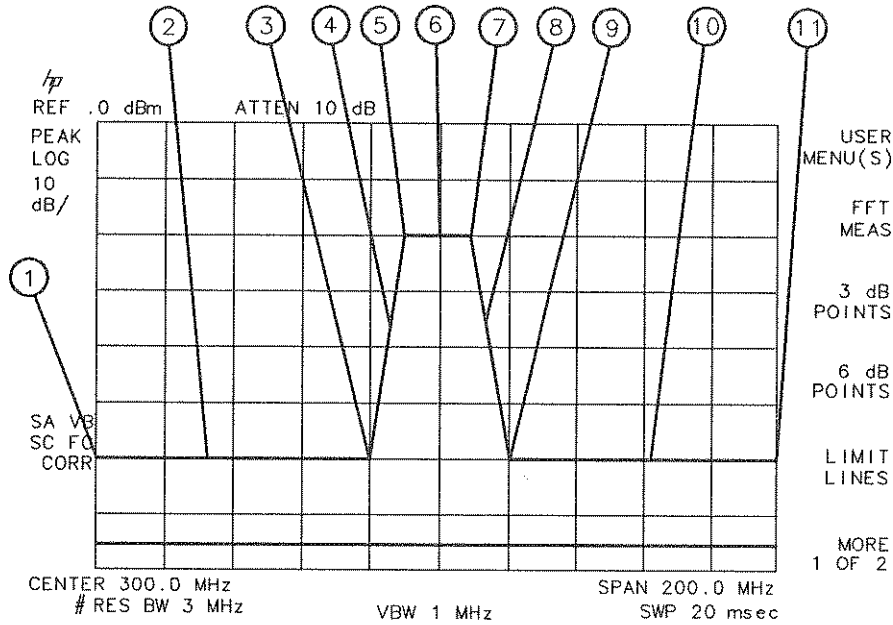
Figure 5-9. Limit-Line Segments
