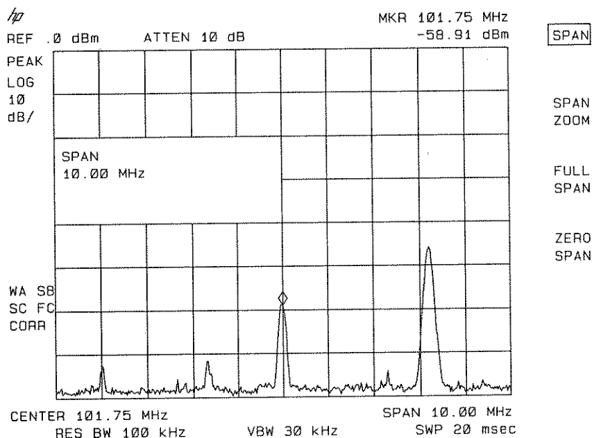
Figure 6-16. Low-Level Signal
