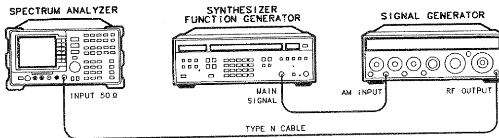
Figure 4-9. Sweep Time Accuracy Test Setup
