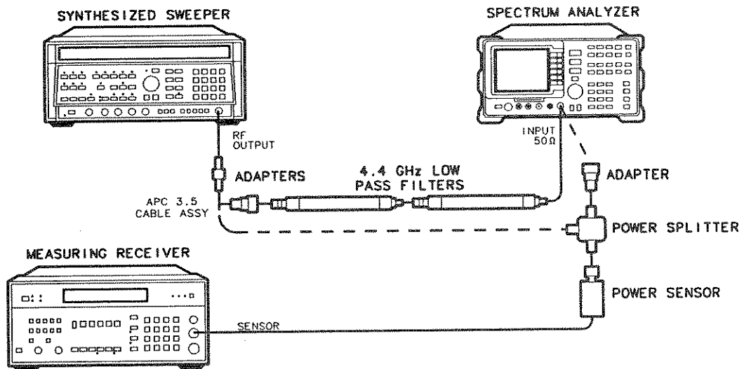
Figure 4-20. Second Harmonic Distortion Test Setup, >2.9 GHz
