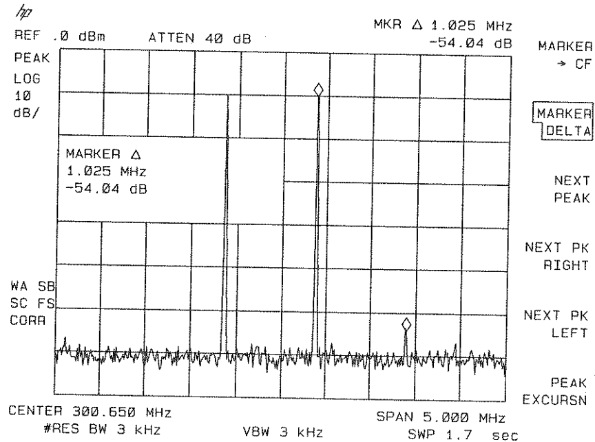
Figure 6-25. Measuring the Distortion Product
