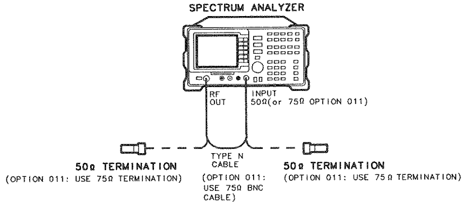
Figure 3-31. Tracking Generator Feedthrough Test Setup
